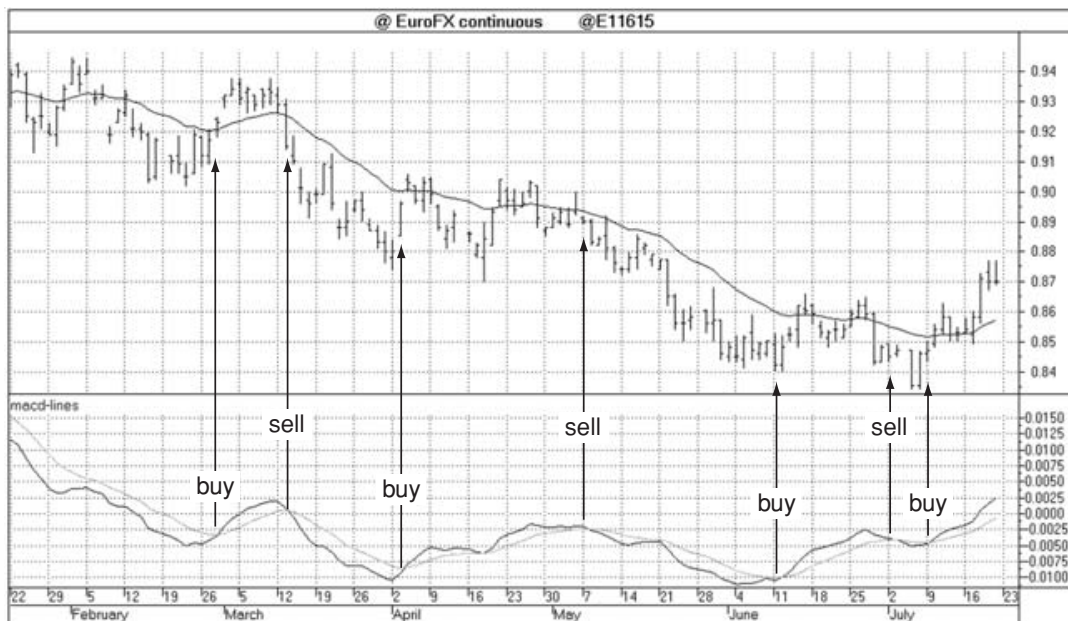
Figure 5.8 MACD Lines
