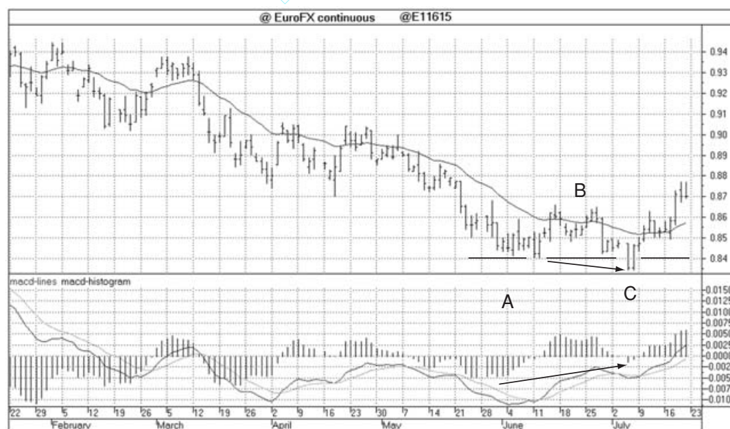
Figure 5.9 MACD-Histogram
